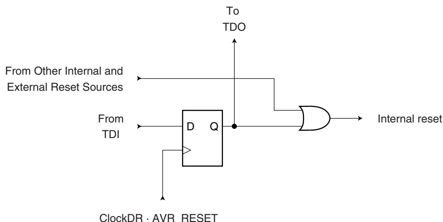
Figure 27-2. Reset Register
