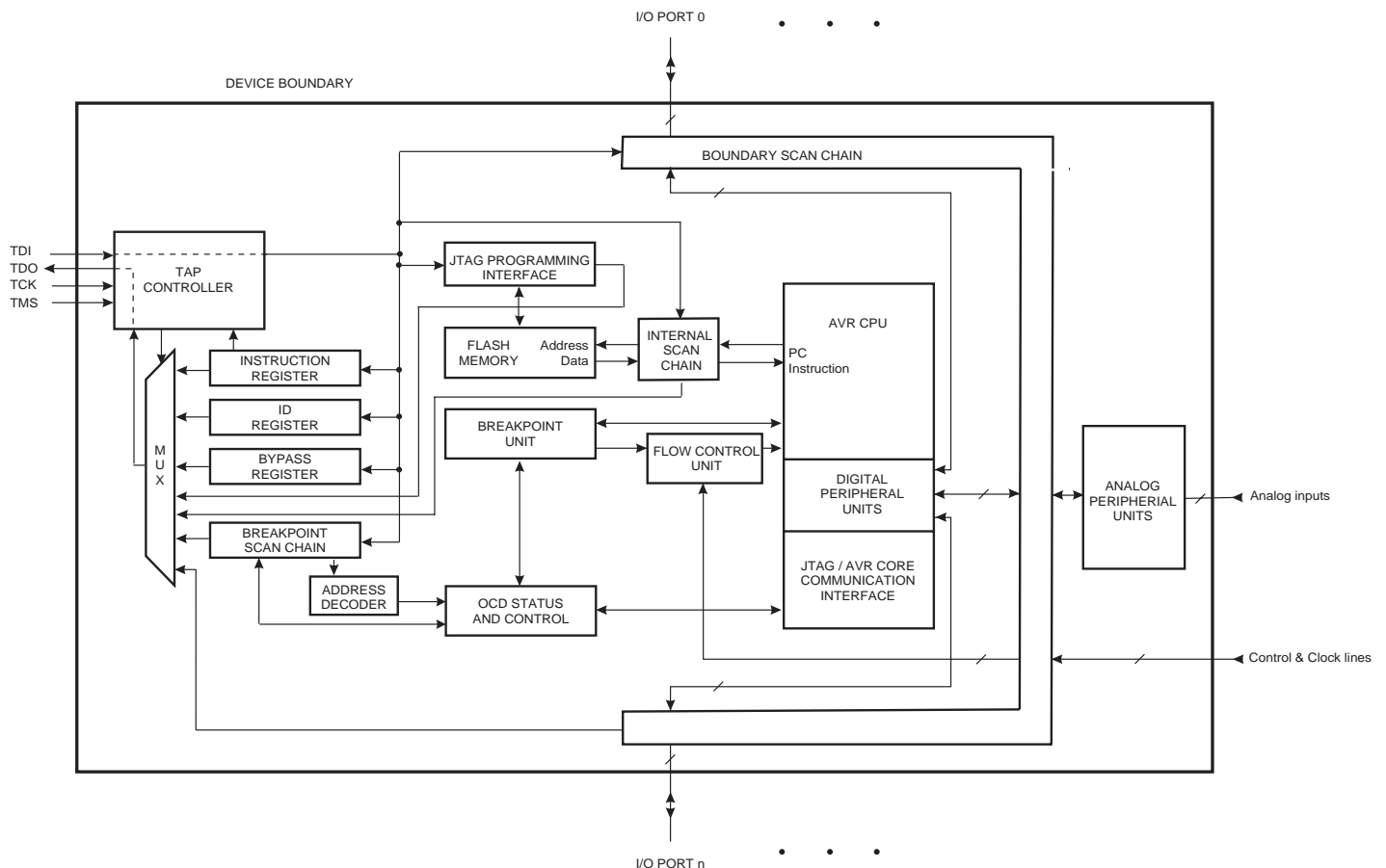
Figure 26-1. Block Diagram
