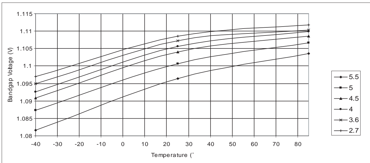
Figure 31-16. Bandgap voltage vs. Temperature
