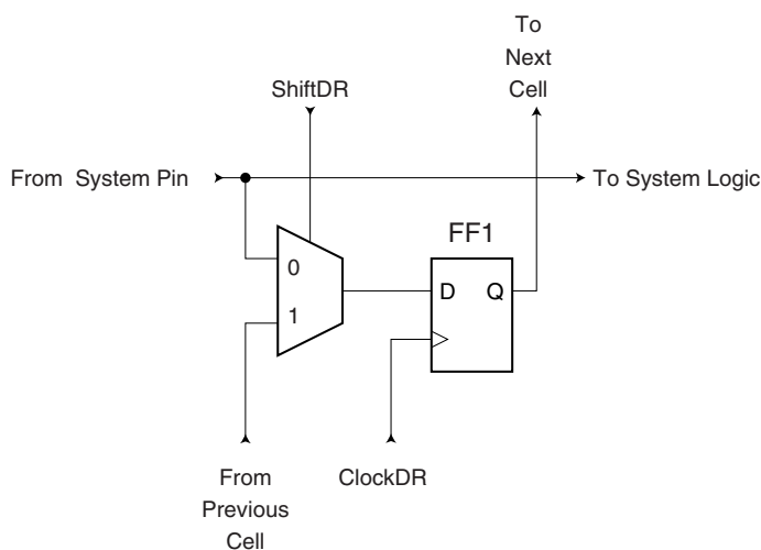
Figure 27-5. Observe-only Cell
