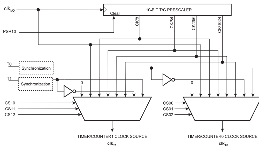
Figure 13-9. Prescaler for Timer/Counter0 and Timer/Counter1 (1)
