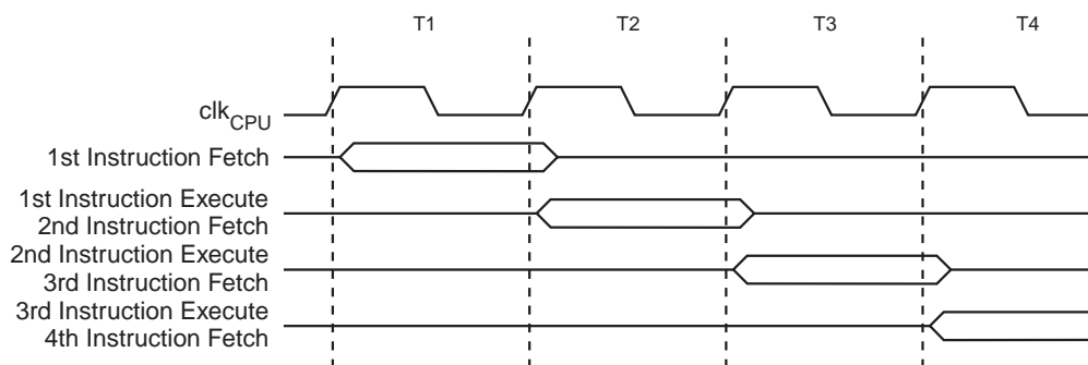
Figure 2. The Parallel Instruction Fetches and Instruction Executions
