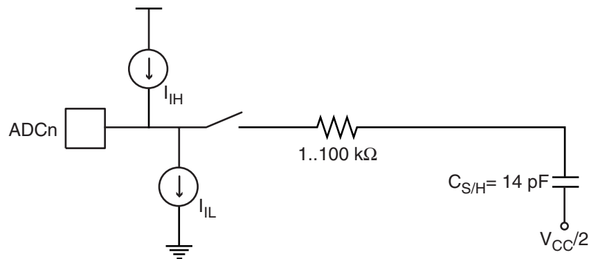
Figure 20-8. Analog Input Circuitry
