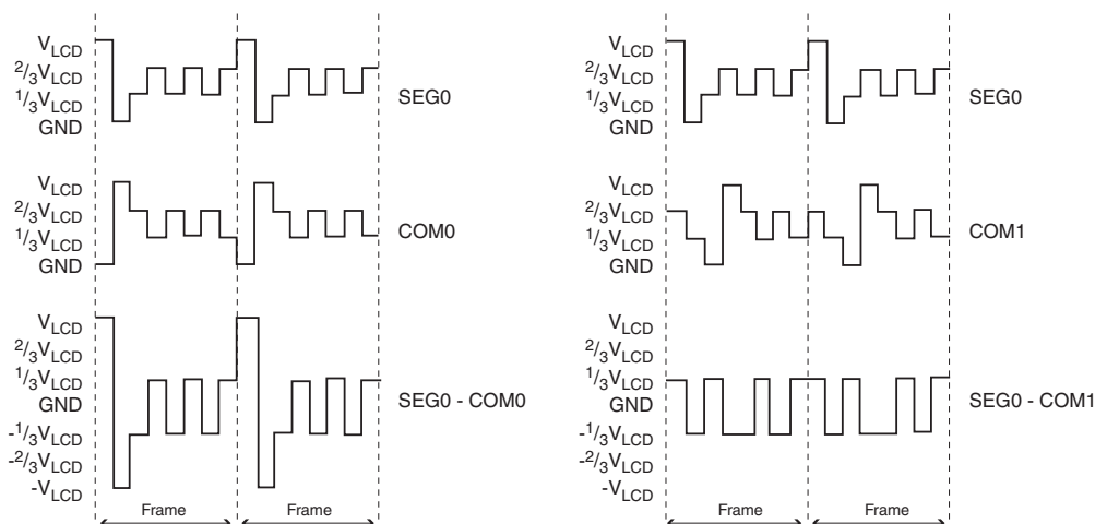
Figure 21-6. Driving a LCD with Four Common Terminals
