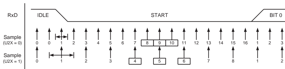
Figure 17-6. Start Bit Sampling
