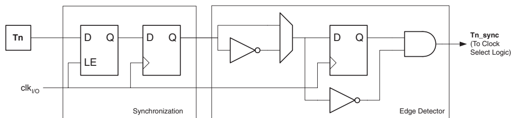
Figure 13-8. T1/T0 Pin Sampling
