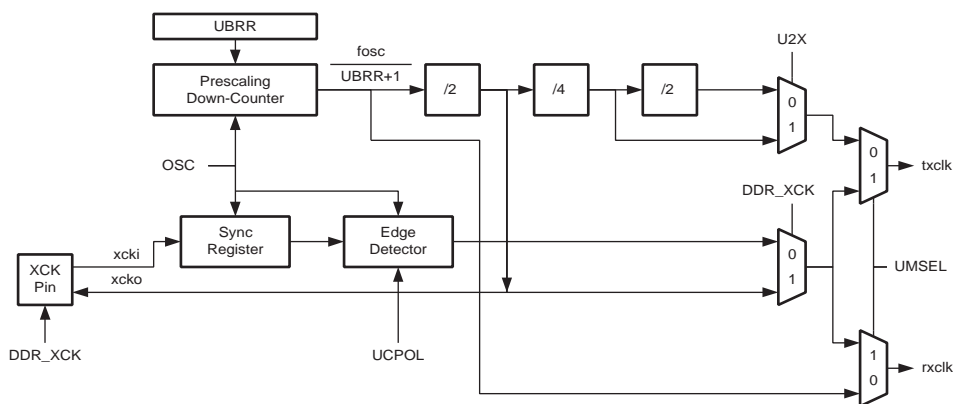
Figure 17-2. Clock Generation Logic, Block Diagram
