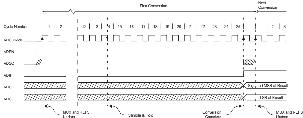
Figure 20-5. ADC Timing Diagram, Single Conversion
