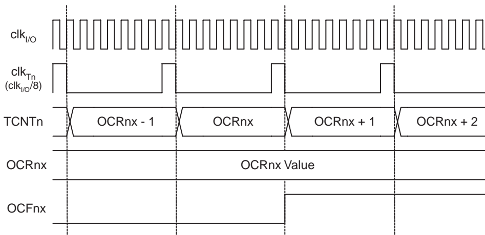
Figure 15-10. Timer/Counter Timing Diagram, Setting of OCF2A, with Prescaler ( f_{clk\_I/O}/8 )
