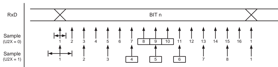
Figure 17-7. Sampling of Data and Parity Bit
