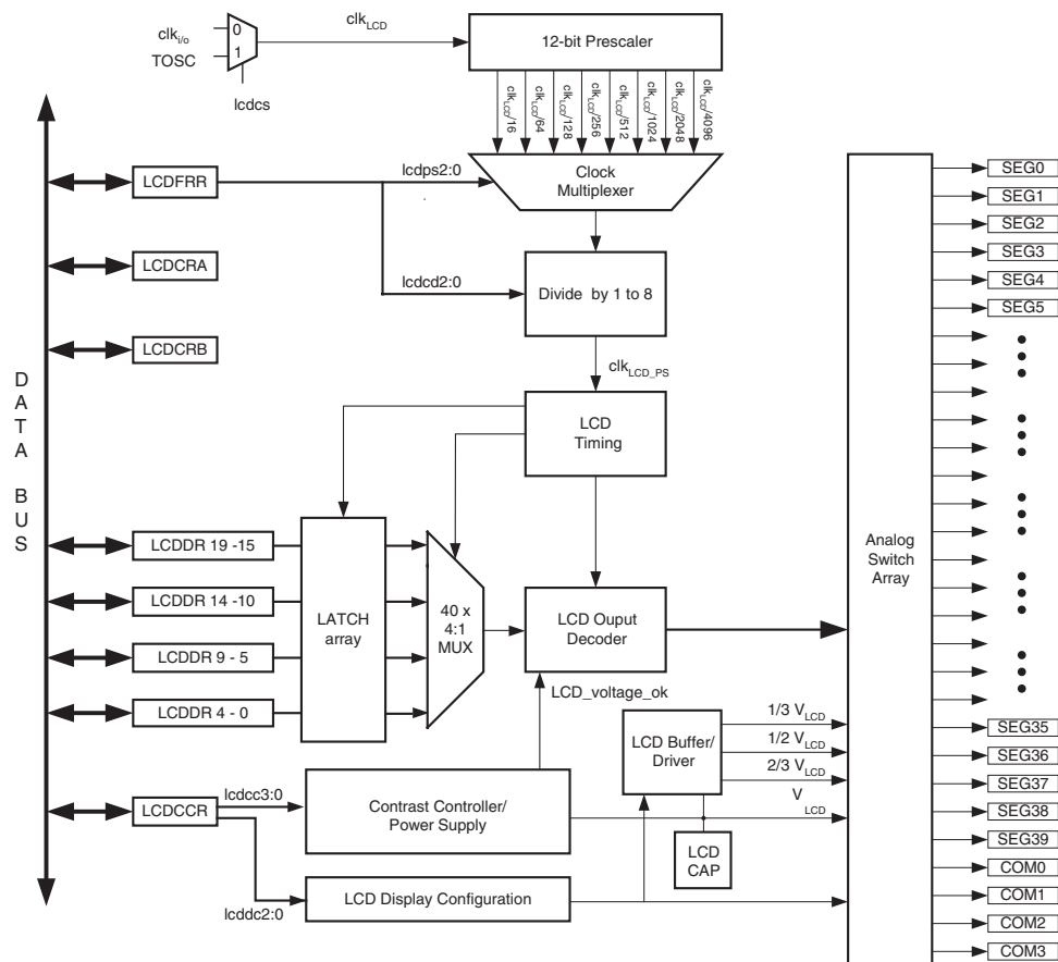
Figure 21-1. LCD Module Block Diagram
