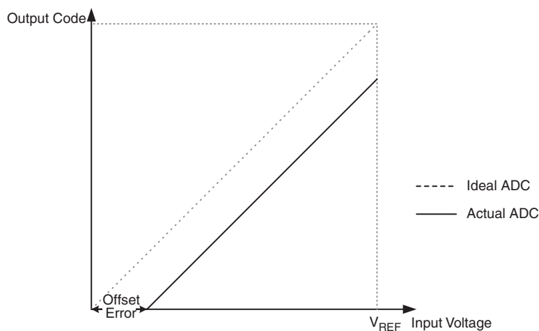
Figure 20-10. Offset Error
