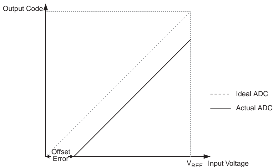
Figure 24-11. Offset Error
