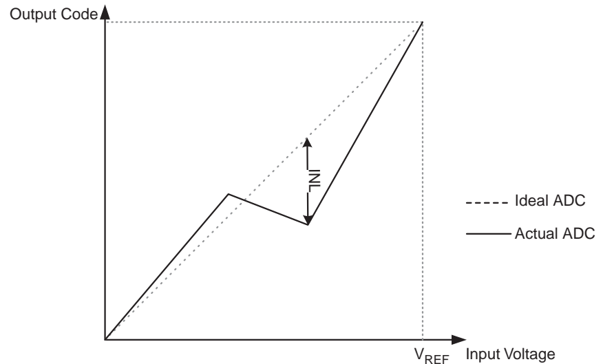
Figure 24-13. Integral Non-linearity (INL)
