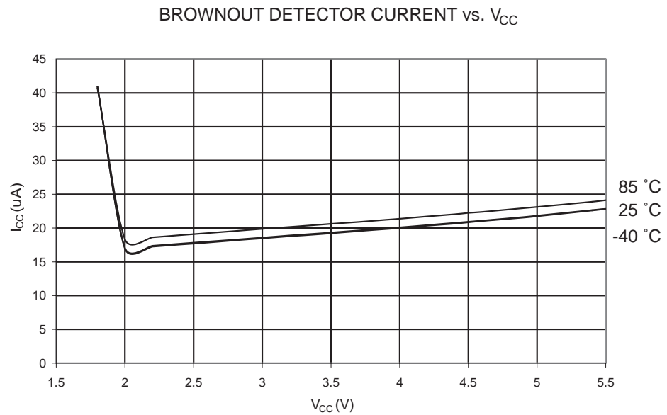
Figure 23-38. Brownout Detector Current vs. V_{CC}
