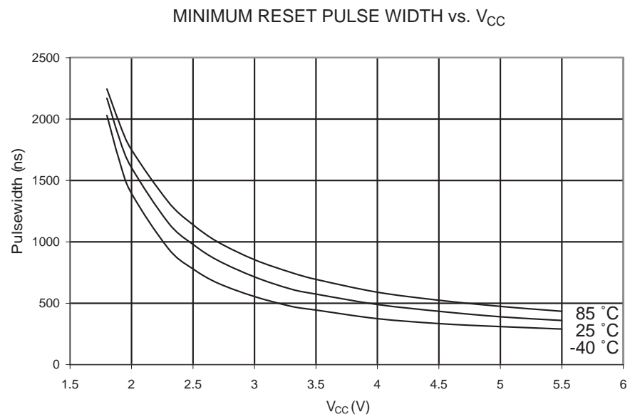
Figure 23-41. Minimum Reset Pulse Width vs. V_{CC}
