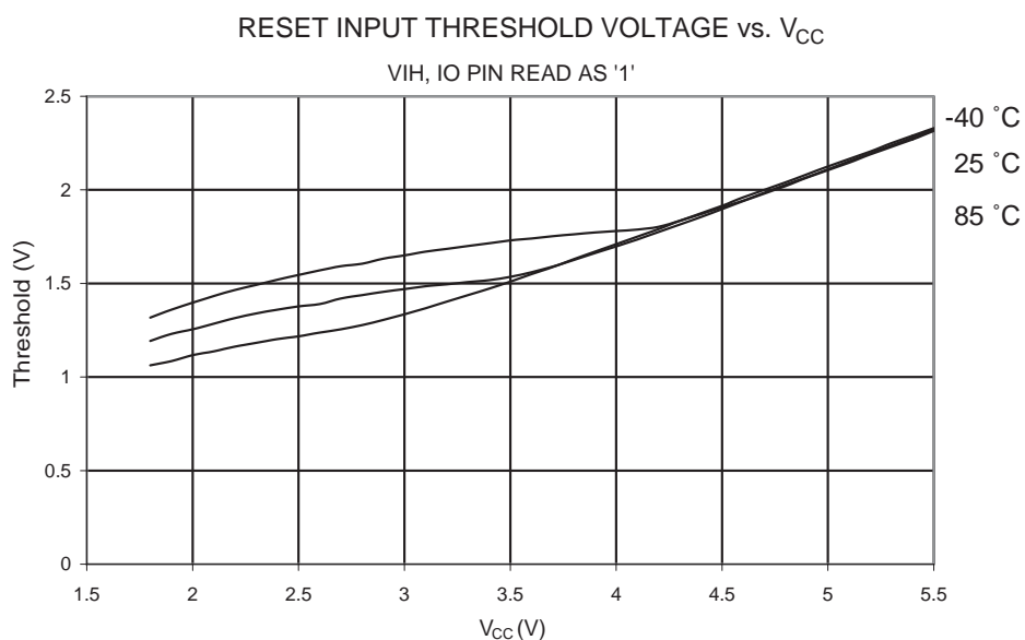
Figure 23-27. Reset Input Threshold Voltage vs. V_{CC} ( V_{IH} , IO Pin Threshold as '1')
