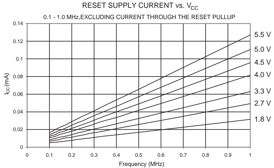
Figure 23-39. Reset Supply Current vs. V_{CC} (0.1 - 1.0 MHz, excluding Current Through the Reset Pull-up)
