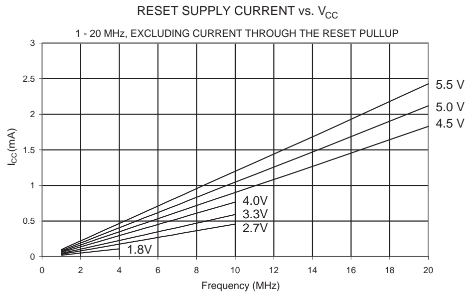
Figure 23-40. Reset Supply Current vs. V_{CC} (1 - 20 MHz, Excluding Current Through the Reset Pull-up)
