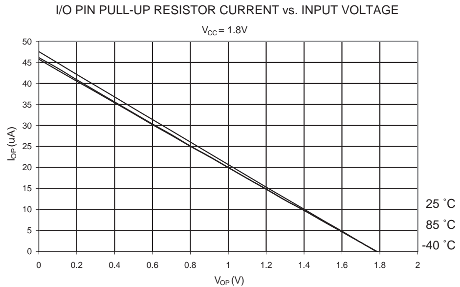
Figure 23-14. I/O pin Pull-up Resistor Current vs. Input Voltage ( V_{CC} = 1.8V )
