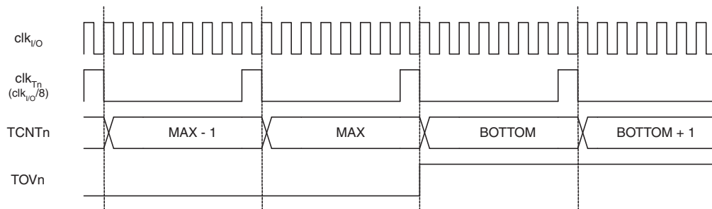
Figure 12-9. Timer/Counter Timing Diagram, with Prescaler ( f_{clk\_I/O}/8 )
