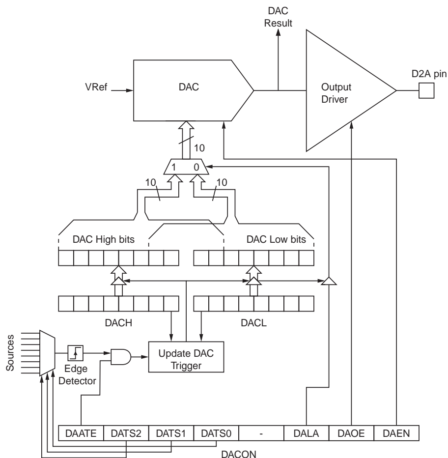
Figure 21-1. Digital to Analog Converter Block Schematic
