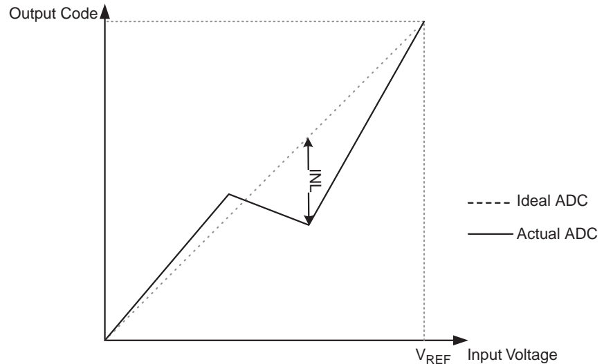
Figure 18-11. Integral Non-linearity (INL)
