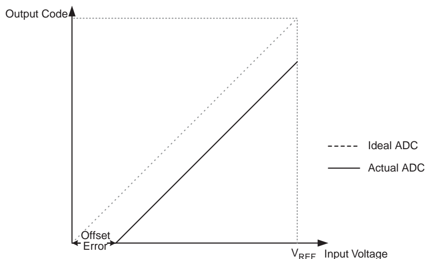
Figure 18-9. Offset Error
