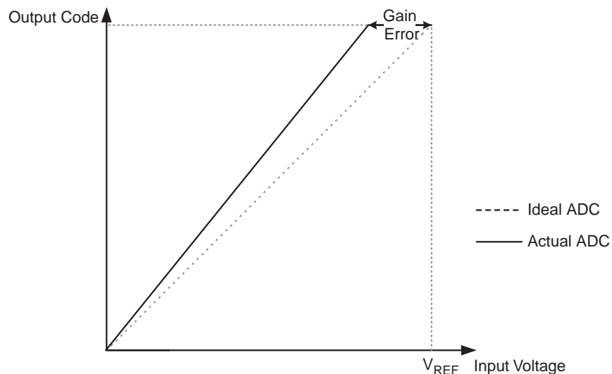
Figure 18-10. Gain Error
