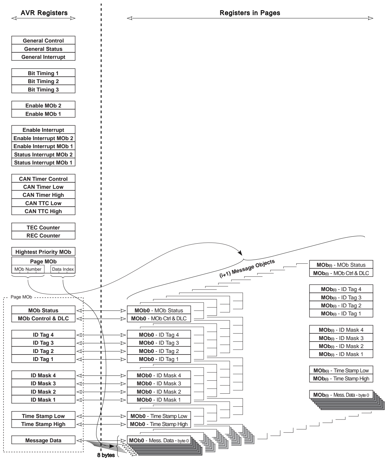
Figure 16-15. Registers Organization
