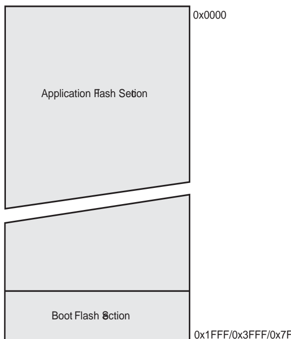
Figure 4-1. Program Memory Map Program Memory
