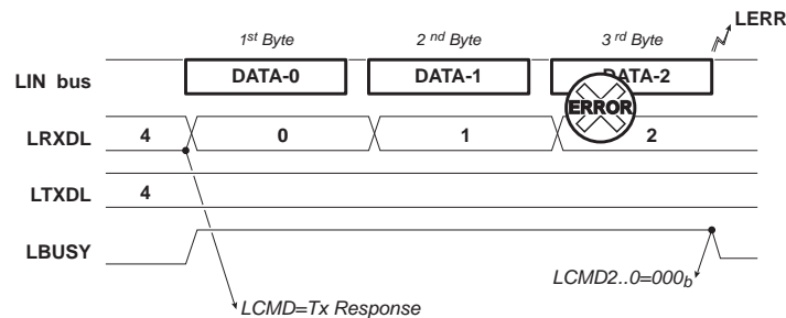
Figure 17-11. Tx Response - Error
