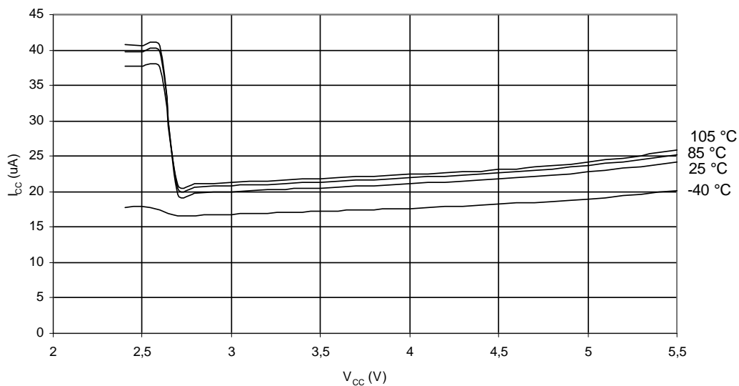
Figure 27-40. ADC Current vs. V_{CC} (ADC at 50 kHz)
