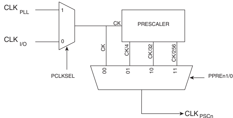
Figure 14-14. Clock selection
