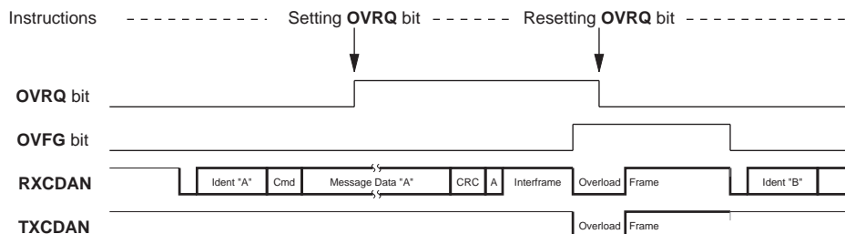
Figure 16-9. Overload Frame
