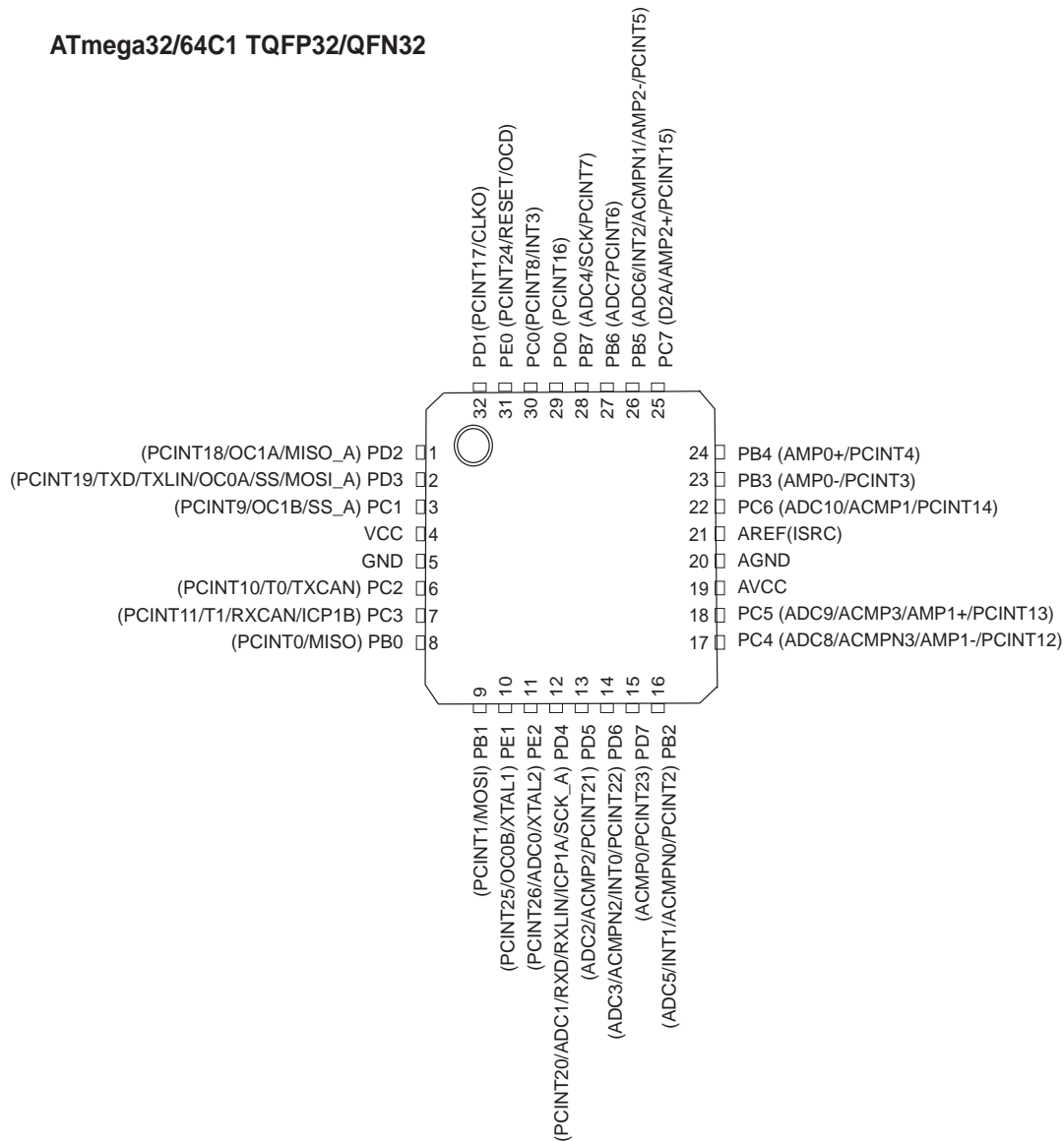
Figure 1-2. ATmega32/64C1 TQFP32/QFN32 (7*7 mm) Package
