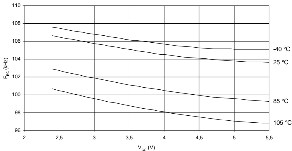
Figure 27-36. Calibrated 8 MHz RC Oscillator Frequency vs. Temperature
