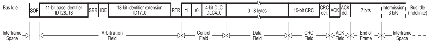
Figure 16-2. CAN Extended Frames
