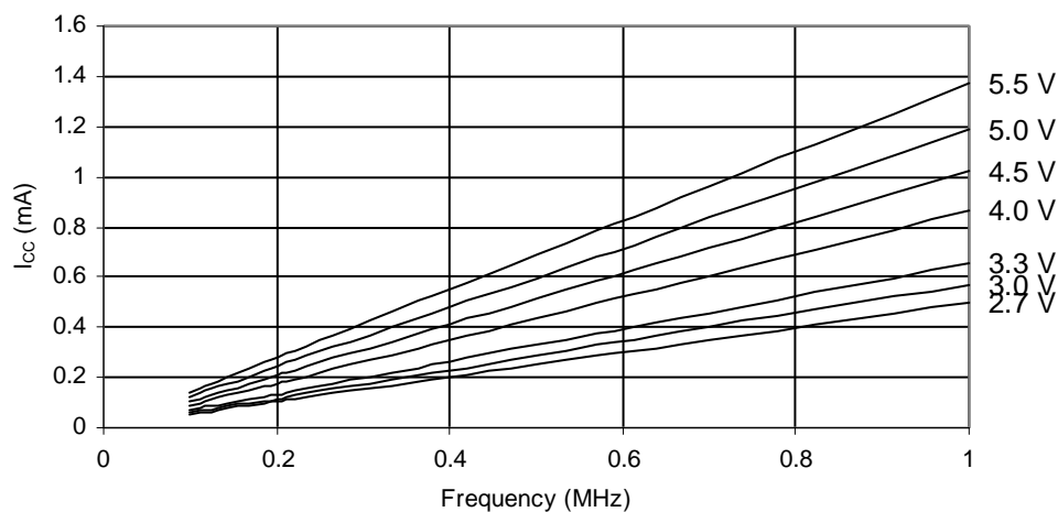
Figure 27-2. Active Supply Current vs. Frequency (1 - 24 MHz)
